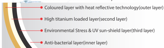
Cross-section of 'Waterwell Wonder 4 Layer' water tank
